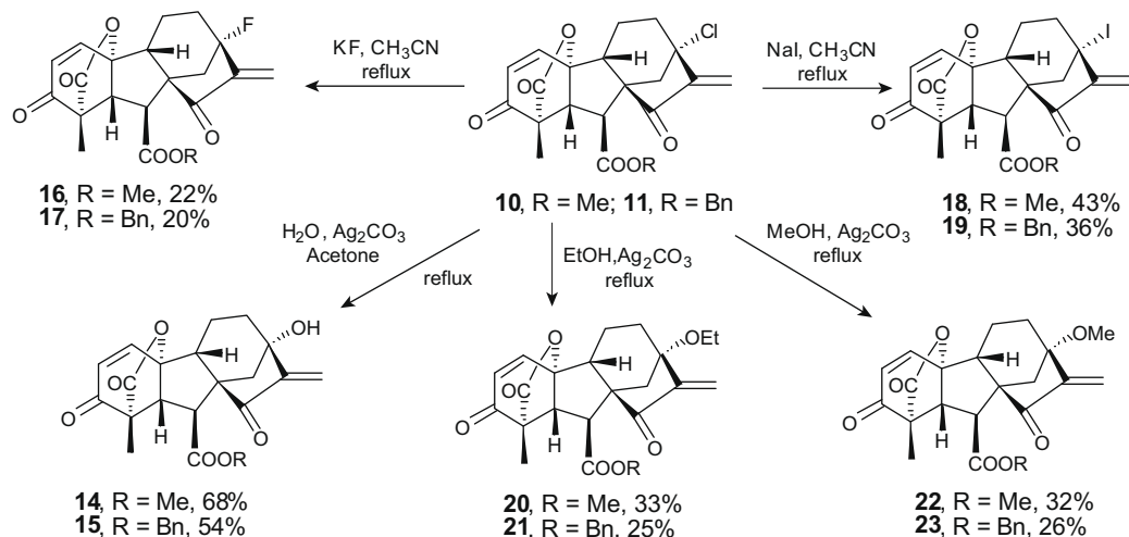
Scheme 3. Synthesis of new gibberellin derivatives bearing \alpha,\beta -unsaturated ketone moiety.
